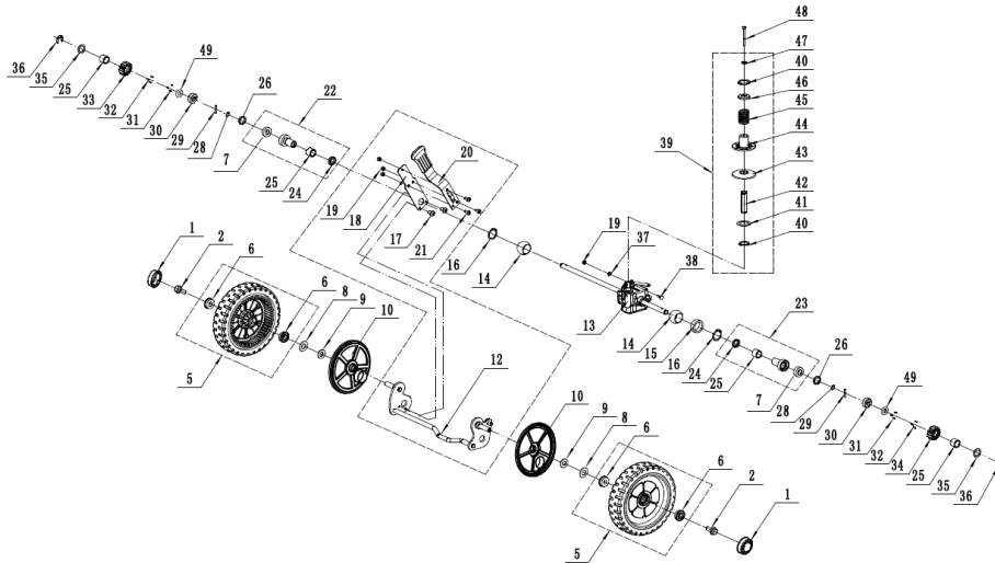
FIG.5 Rear Axle
